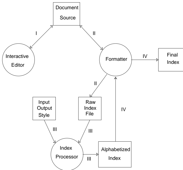
Figure 1: Circles in the picture represent processors, squares are documents or auxiliary files. In Step I, the author uses an editor to place index commands in the document. In Step II, a raw index is generated as a by-product of formatting. In Step III, this raw index together with some optional style information are taken as input to the index processor and an alphabetized version is created. Finally in Step IV, the index is formatted to yield the ultimate result.
